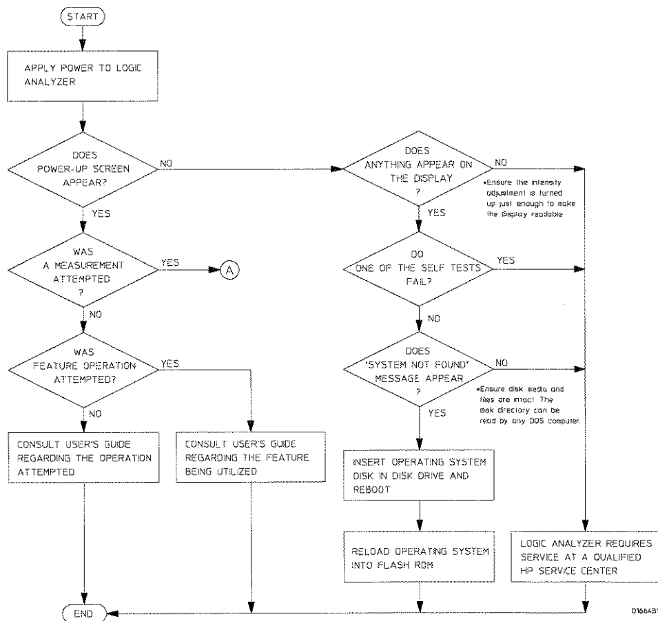
Troubleshooting Flowchart 1
