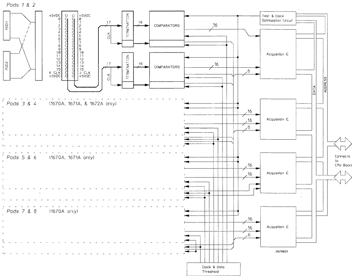
Logic acquisition board
